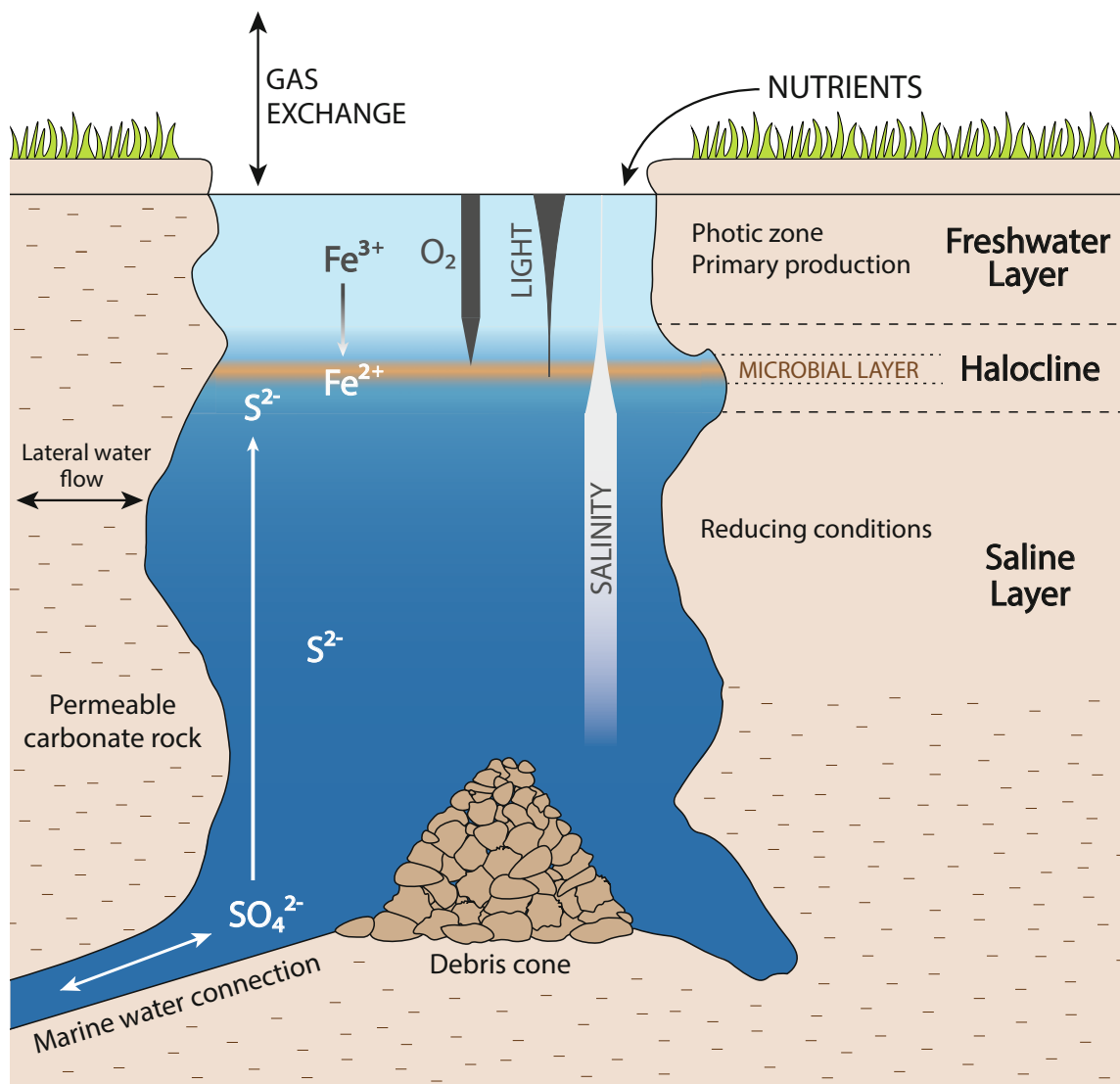
Fig. 1. Schematic figure of a blue hole including relevant physical and chemical characteristics and the possibility of deep passageways. The debris cone is a common feature in blue holes, it is created from falling debris and can vary in size and shape.
